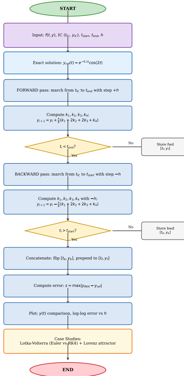
Figure 10.3: Algorithm flowchart: bidirectional RK4 integration and nonlinear case studies.
