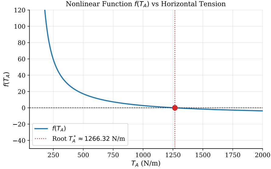
Figure 6.1: f(T_A) versus horizontal tension T_A . The unique root is visible as a zero crossing near T_A \approx 1266 N/m [4].
