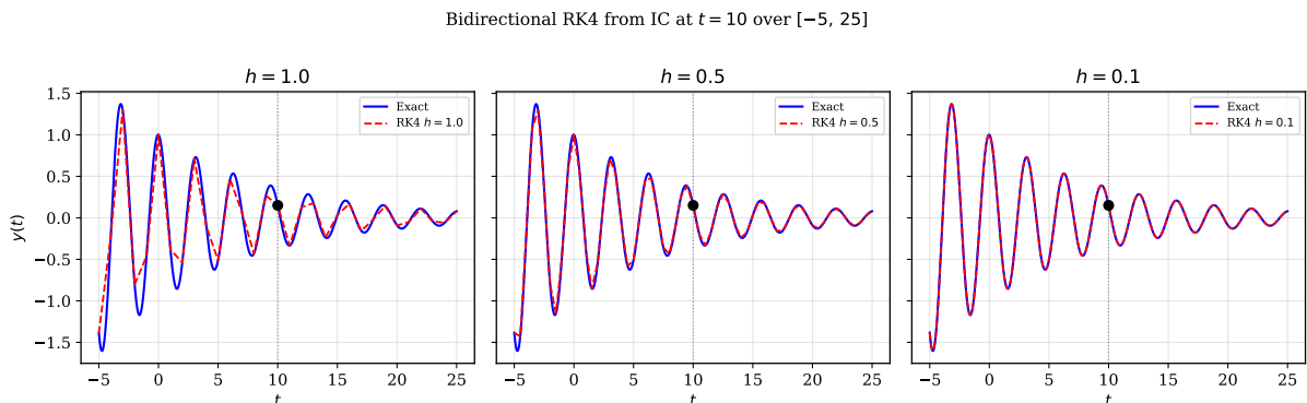
Figure 10.4: Bidirectional RK4 (red dashed) versus exact solution (blue) for three step sizes. At h = 1.0 noticeable phase drift accumulates; reducing to h = 0.1 yields near-perfect agreement across the entire domain [-5, 25] .
