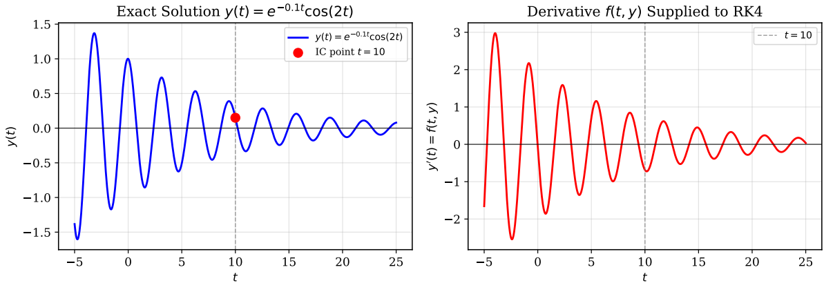
Figure 10.2: Left: exact solution y(t) = e^{-0.1t} \cos(2t) over [-5, 25] ; the red dot marks the interior IC at t = 10 . Right: the corresponding derivative f(t, y) supplied to the RK4 integrator.
